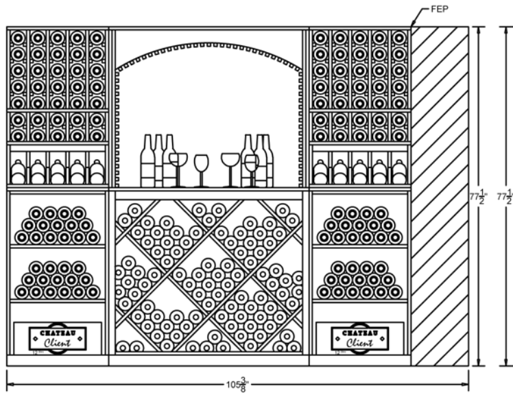
ELEVATION -A-
