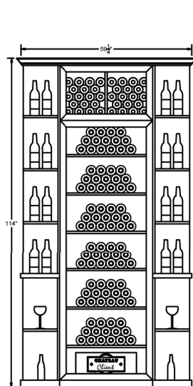
ELEVATION -C- QTY. 2 REQ.
