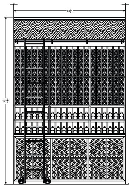
ELEVATION -A-
